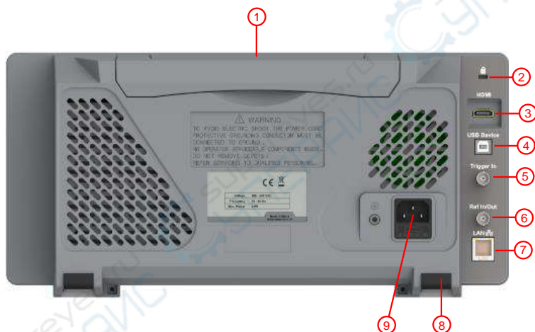
Figure 4-6 Rear Panel
